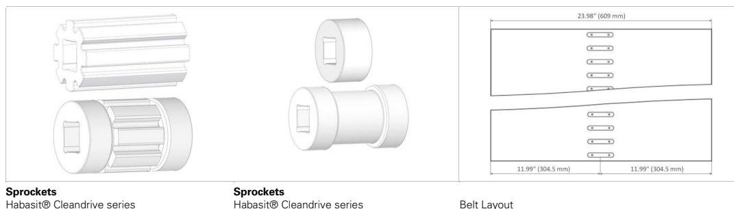
Belt Layout
