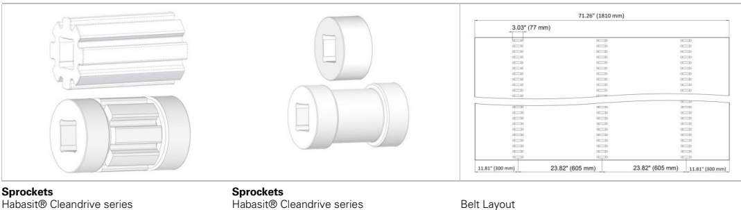
Belt Layout
