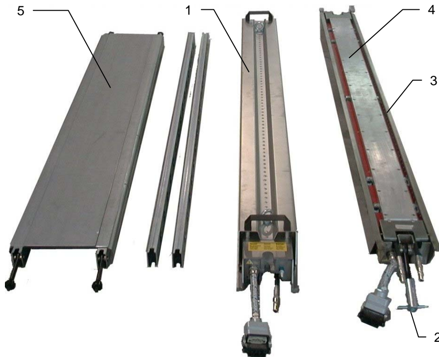
FIGURE 4 - MAIN ELEMENTS OF THE PM-1606
