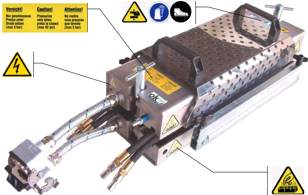
FIGURE 2 - POSITION OF SIGNS ON THE PRESS
