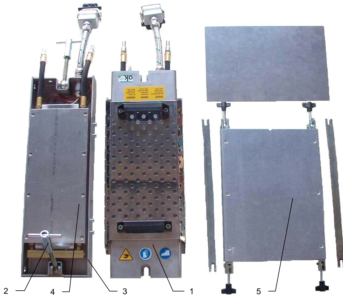
FIGURE 4 - MAIN ELEMENTS OF THE PM-306/160
