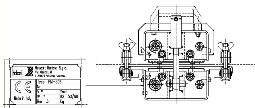
FIGURE 1 - MACHINE IDENTIFICATION PLATE
