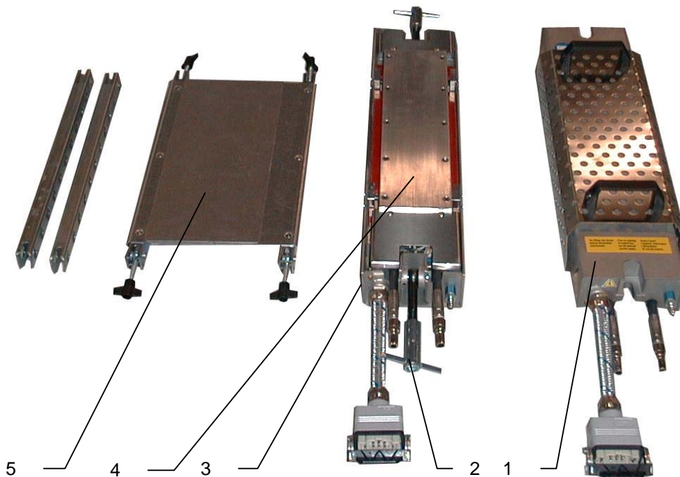
FIGURE 4 - MAIN ELEMENTS OF THE PM-306
