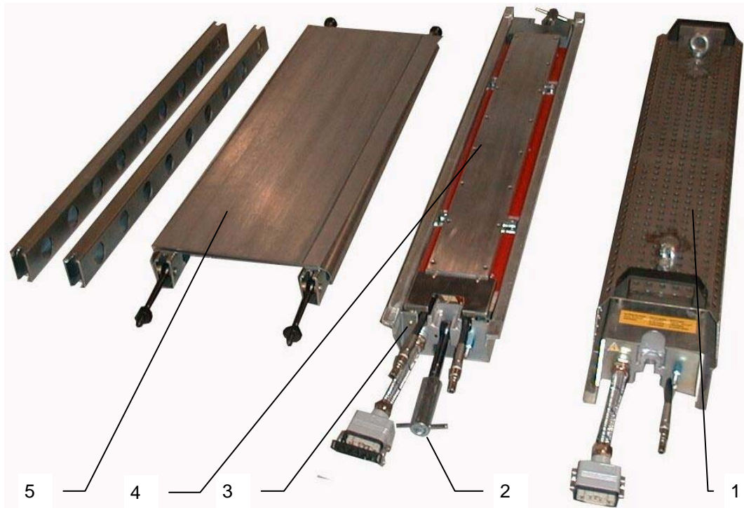
FIGURE 4 - MAIN ELEMENTS OF THE PM-806
