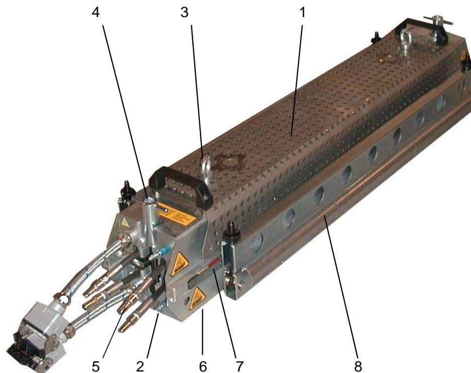
FIGURE 3 - VIEW OF PM-806
