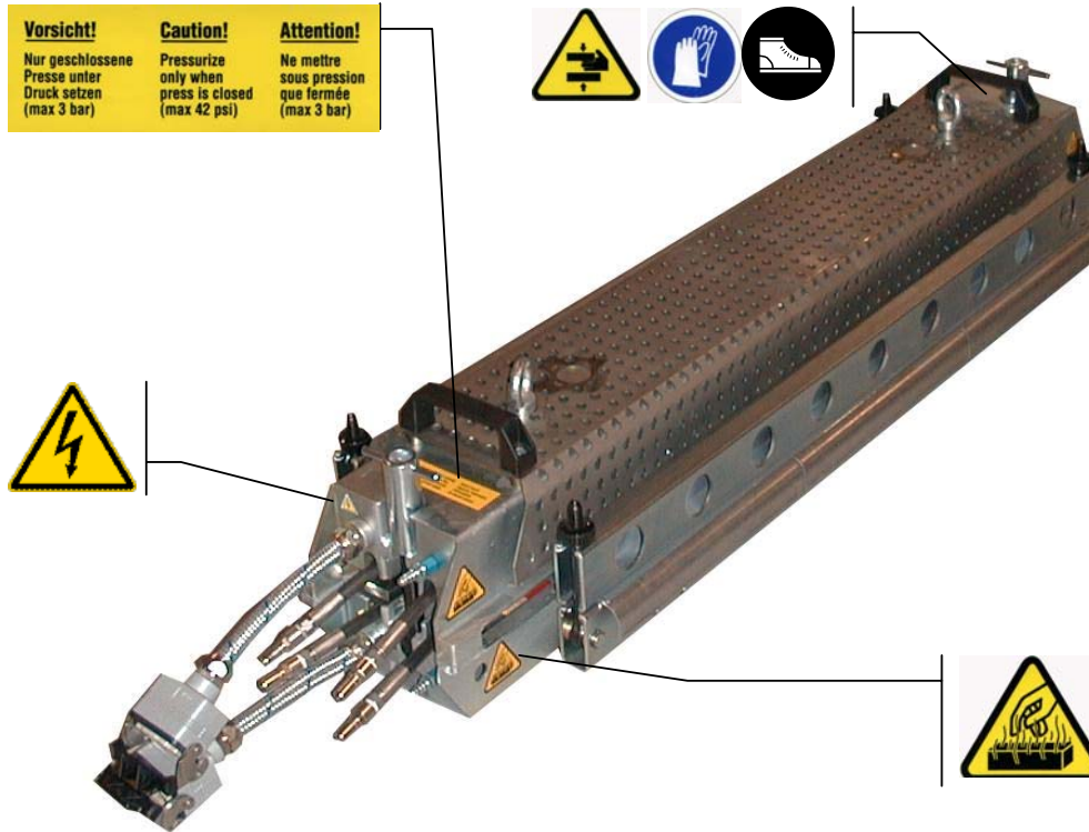
FIGURE 2 - POSITION OF SIGNS ON THE PRESS
