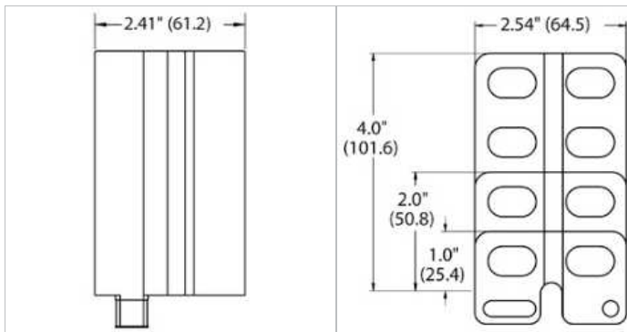
Side guards Side guards are available in 1/2", 1", 2" and 4" heights
