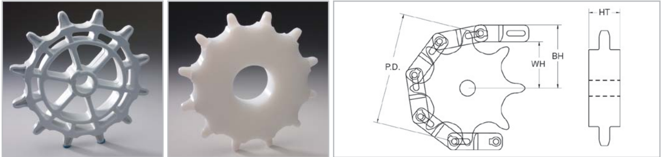
Molded sprocket
