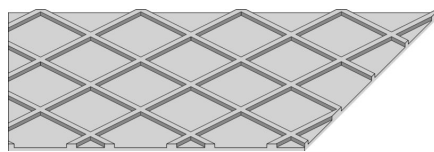
SIM CW
